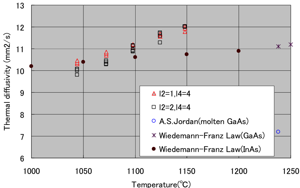
Fig. 5 Thermal diffusivity of molten In 0.8 Ga 0.2 As
