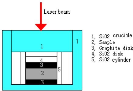
Fog.2 Quartz container
