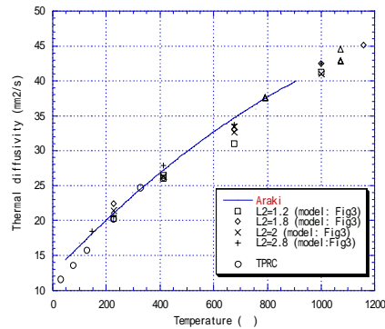
Fig.4 Thermal diffusivity of molten Ga
