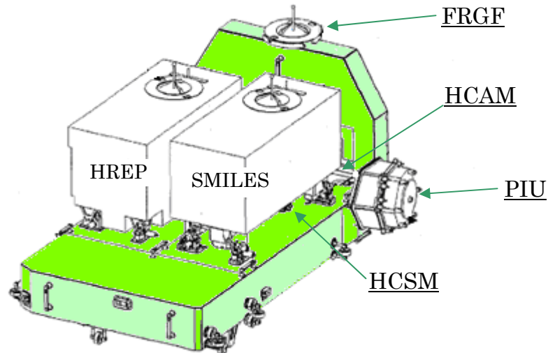
Fig. 1.2.3-3 Exposed Pallet for EF Payload (Note: Configuration for the HTV-1 Mission)
