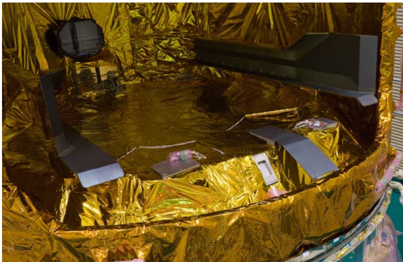
Fig. 1.2.2-4 Enlarged View of the ULC
