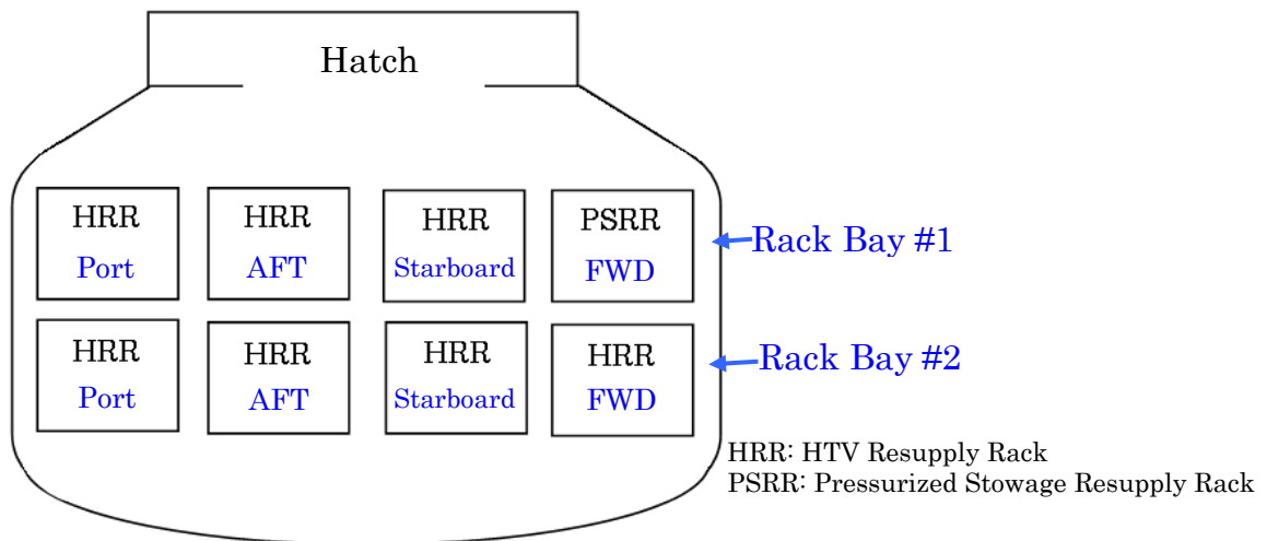
Fig. 1.2.1-3 Rack Layout inside the HTV (HTV-1)
