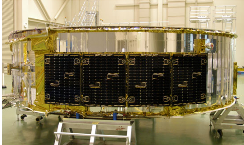
Fig. 1.2.4-1 Avionics Module (Side View)
