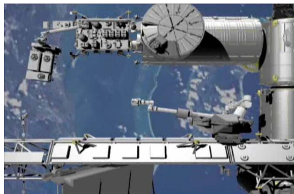
The EP is handed over to Kibo's robotic arm (JEMRMS) and temporarily installed on Kibo's Exposed Facility
