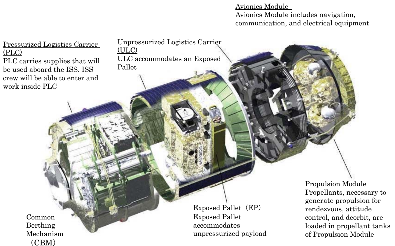
Fig. 1.2-1 HTV Configuration Diagram
