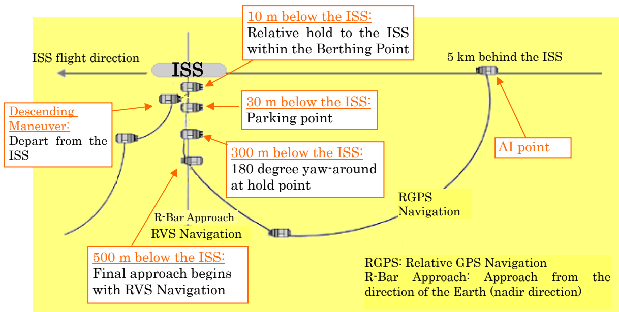
Fig. 1.3.4-1 HTV's RGPS Navigation and R-Bar Approach
