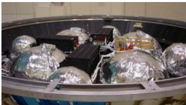
Fig. 1.2.5-2 Enlarged Photo: Propellant Tanks
