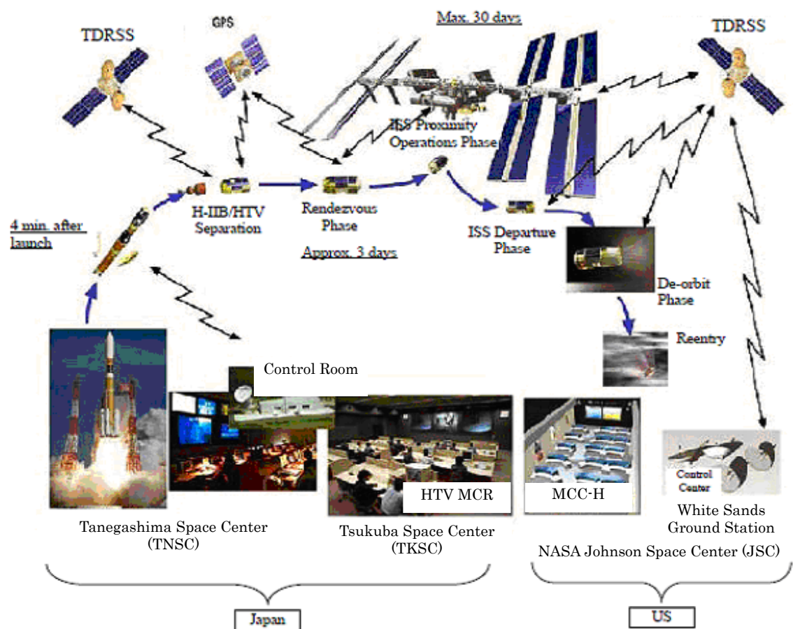
Fig. 1.3-1 HTV Operations
