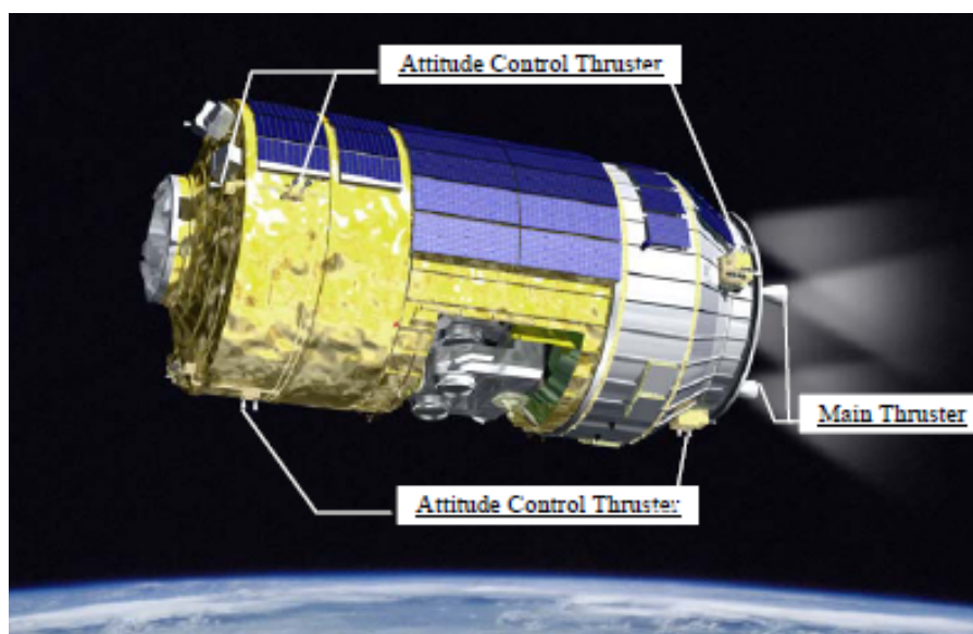
Fig. 1.2.5-5 Approximate Locations of Main Thrusters and Attitude Control Thrusters
