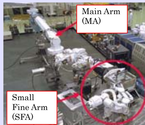
Kibo's Robotic Arm (JEMRMS)
