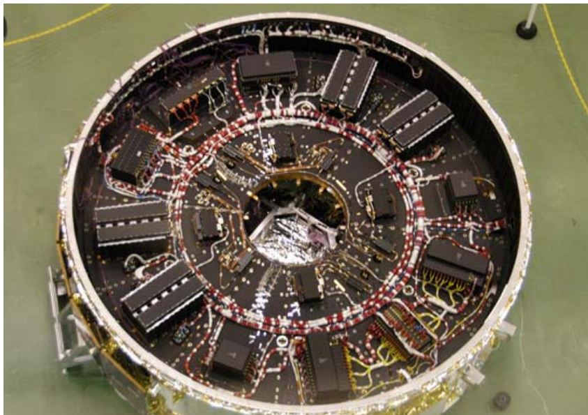
Fig. 1.2.4-2 Avionics Module (Viewed from Above)
