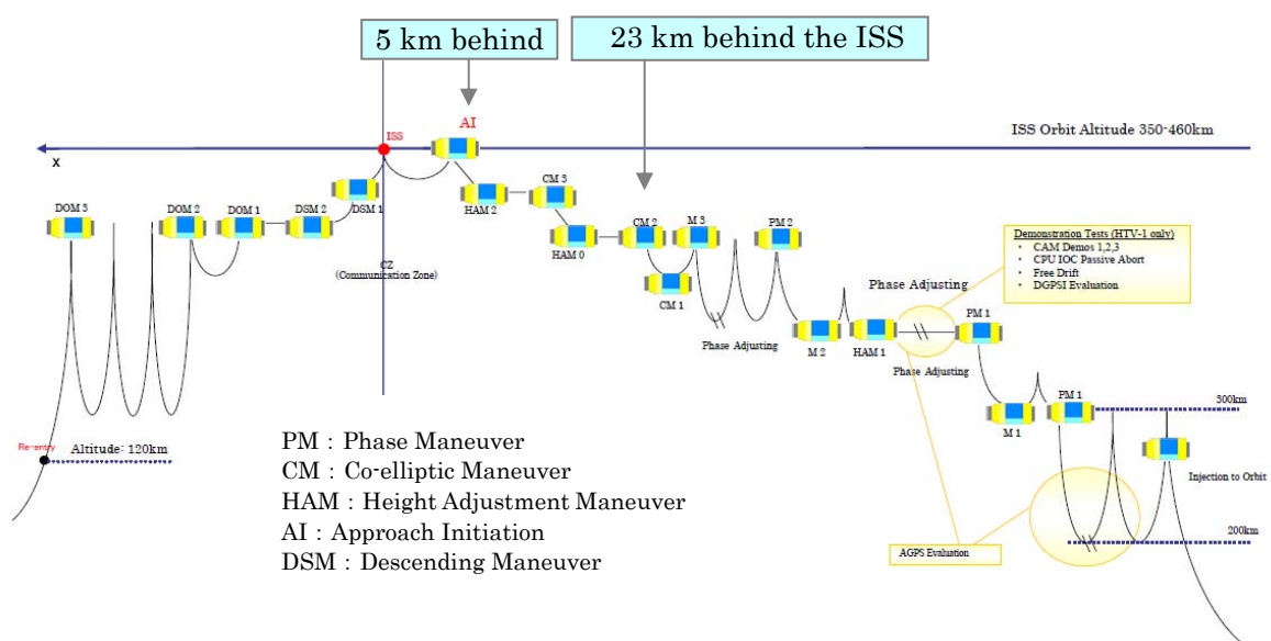
Fig. 1.3.3-1 HTV Rendezvous Profile
