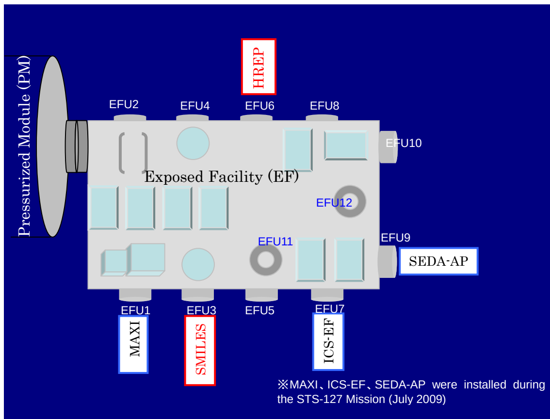
Fig. 2.3.2-4 Attachment Positions of the EF Payloads
