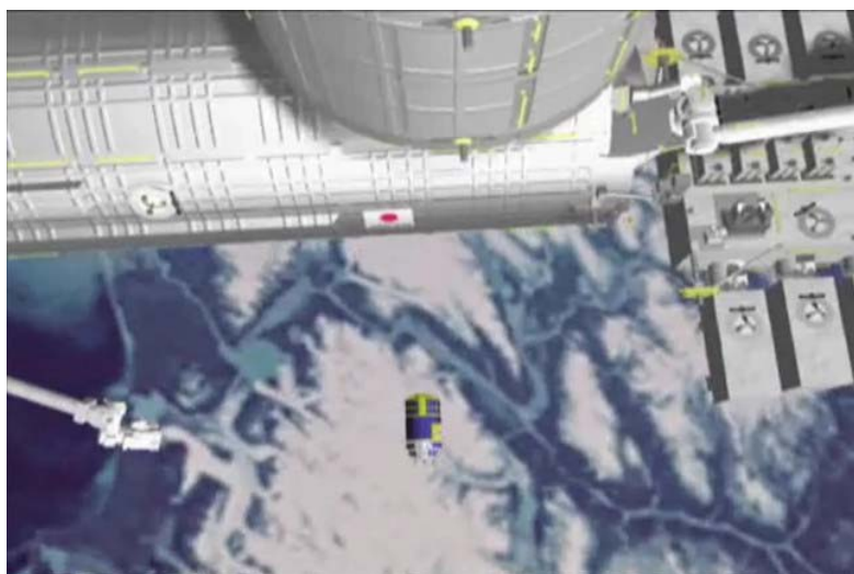
Fig. 1.3.4-2 HTV's Approach (Image)
