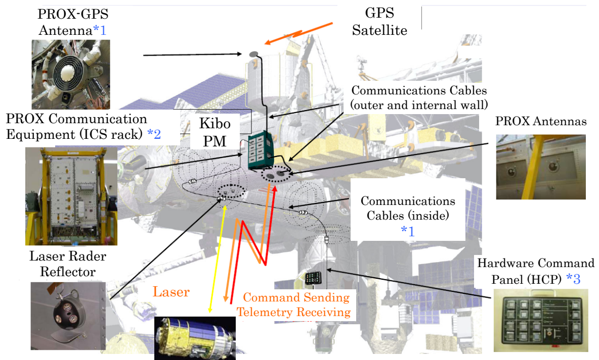
Fig. 1.2.6-1 Locations of the PROX system
