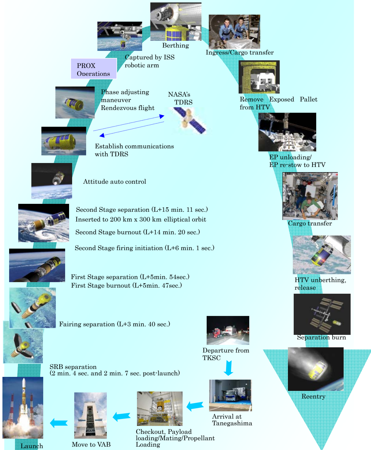
Fig. 2.2-1 HTV-1 Mission Event Sequence
