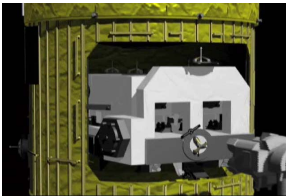
SSRMS removes the EP from the ULC
