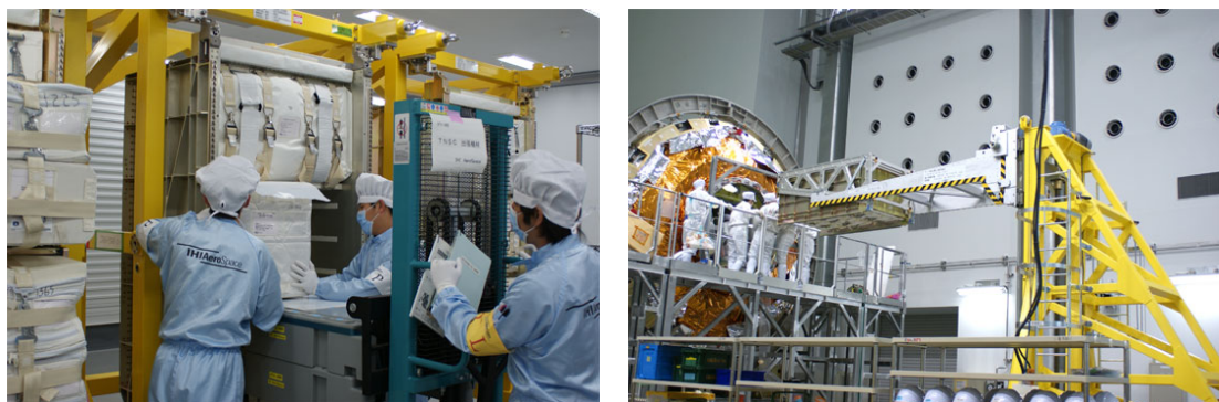
Fig. 1.3.1-1 Cargo Transfer Bags (CTBs) being installed in the HTV Resupply Racks (HRRs) and an HRR being loaded into the PLC (Launch Processing on the HTV-1 Mission)
