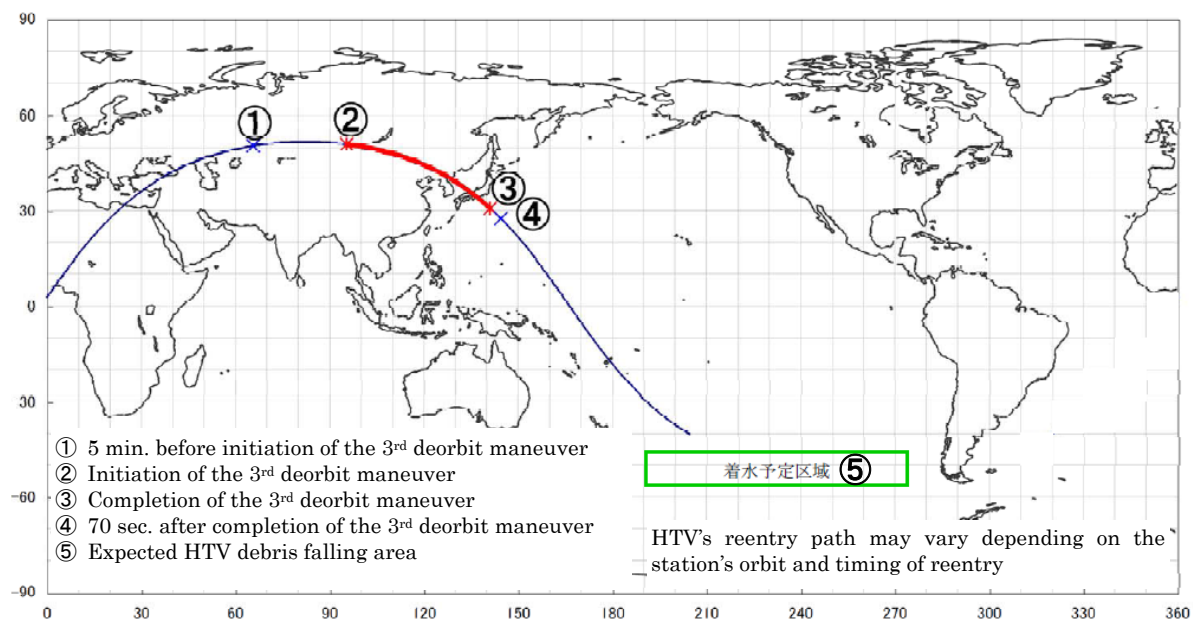
Fig. 1.3.6-2 HTV's Projected Reentry Path (Red Lines) and Expected HTV Debris Falling Area
