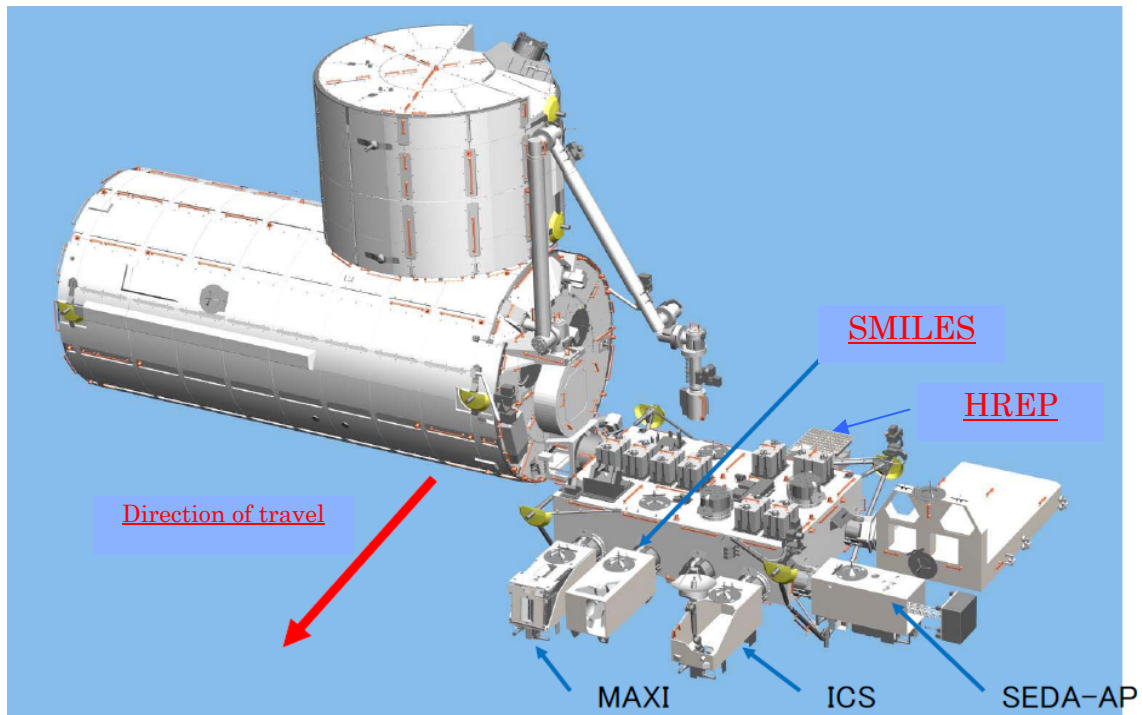
Fig. 2.3.2-3 Attachment Positions of HREP and SMILES
