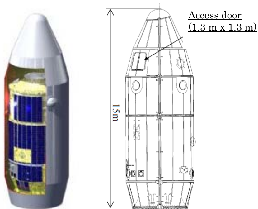
Fig. 1.3.1-5 HTV Installed in H-IIB Rocket Fairing (Image: left) Location of Access Door for HTV Late Access (Image: right)
