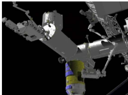
SSRMS removes the EP from the ULC
