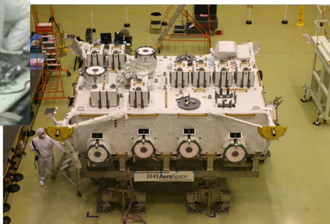
Kibo's Exposed Facility (EF)
