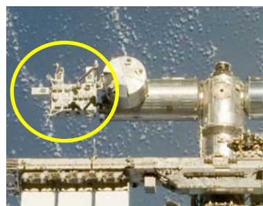
Kibo's EF on the ISS (STS-127)
