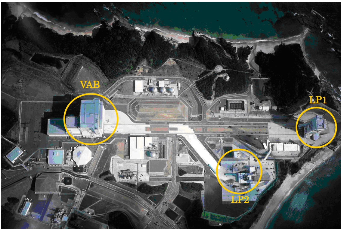
Fig. 1.3.1-9 VAB, Launch Pad 1 (LP1), and Launch Pad 2 (LP2) at the Yoshinobu Launch Complex of TNSC
